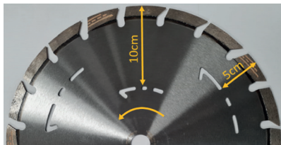
DEPTH OF CUT AND DIRECTION OF ROTATION INDICATOR
